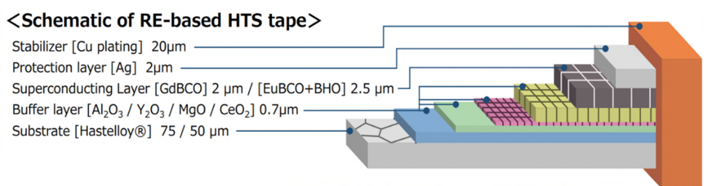
Fig. 3-5-3: Schematic diagram of REBCO tape rod structure
